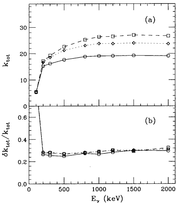
Fig. 4. Panel (a) shows the inferred \gamma multiplicity k_{\text{tot}} as a function of E_\gamma for cascades of twenty \gamma -rays of the same energy. Panel (b) is the FWHM fraction of the k_{\text{tot}} distribution. Three different methods of extracting k_{\text{tot}} are shown: using the 110 Ge and BGO units as elements (solid line and open circles), using 220 elements, by grouping the 110 Ge detectors and their BGO backplugs separately from the other 6 \cdot 110 BGOs (dotted line, diamonds), and by using all 880 separate BGO and Ge detectors as elements (dashed line, squares). The Microball is included in all the above calculations.
