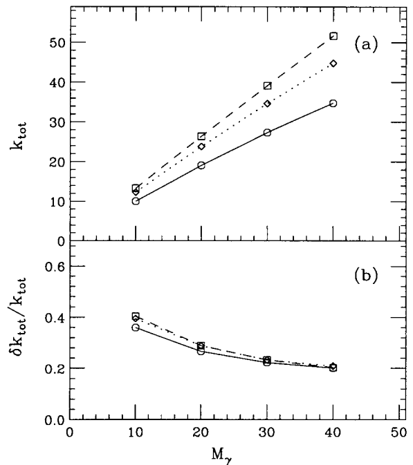
Fig. 5. Panel (a) shows the calculated total \gamma multiplicity as a function of the number of 1 MeV \gamma -rays in a cascade, using the same three methods of extracting k as in Fig. 4. Panel (b) shows the corresponding widths of the k_{\text{tot}} distribution. The Microball is included.
